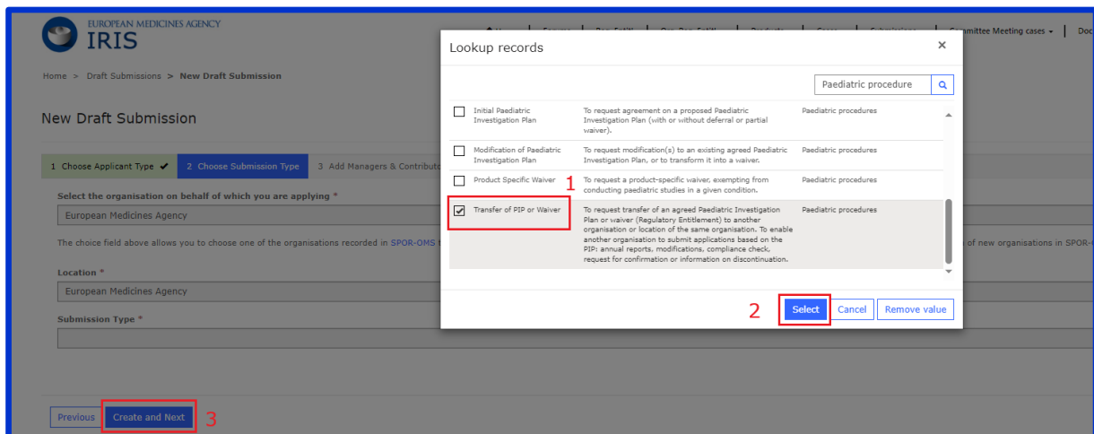
Figure 117: Lookup records
