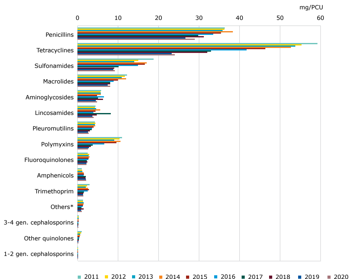
Figure 24. Changes in aggregated sales (mg/PCU) by antimicrobial class in 25 EU/EEA countries 1 , from 2011 to 2020
